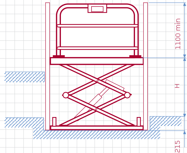
With enclosures/Aluminium-Schacht
